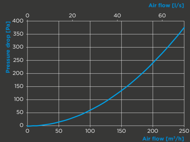
AIR FLOW
